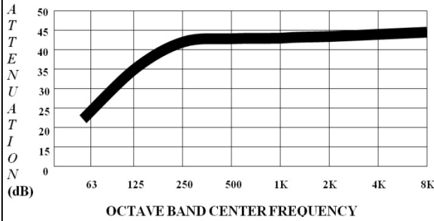
GE6HP TYPICAL ATTENUATION CURVE
